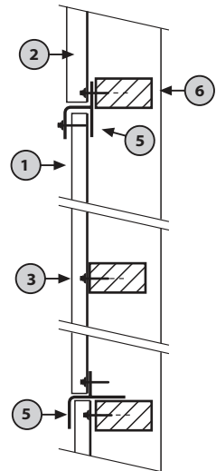
Typical Side Light Vertical Section
